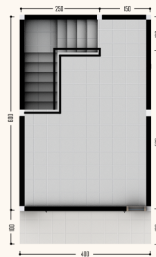
DENAH RUKO LT II
