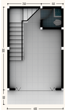
DENAH RUKO LTI
